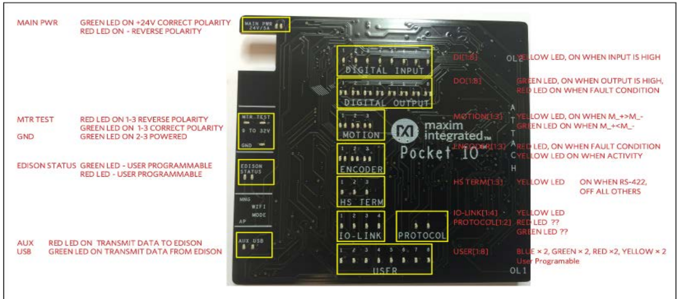
Figure 4. Pocket IO LEDs.
