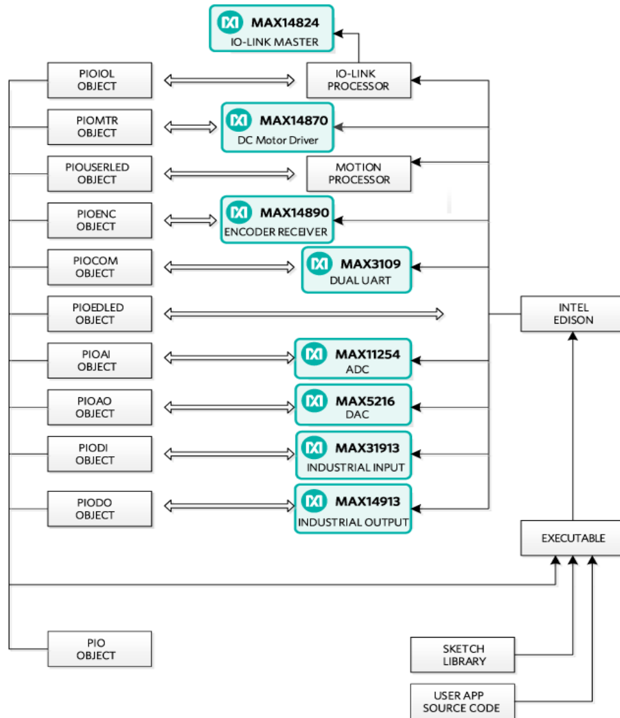
Figure 5. Pocket IO software architecture.
