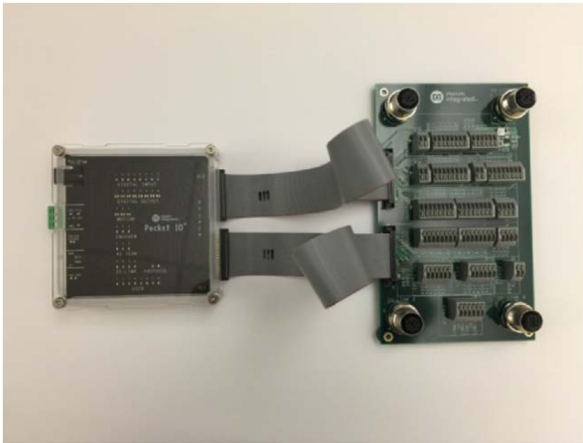
Figure 8. Pocket IO Connected to MAXREFDES150ATACH#.
