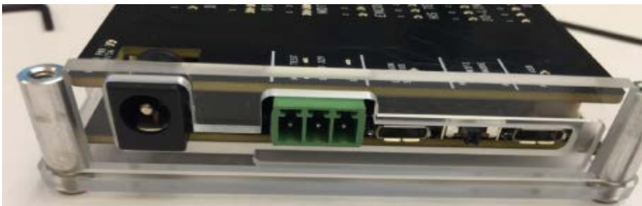
Figure 2. MAXREFDES150# power inputs.
