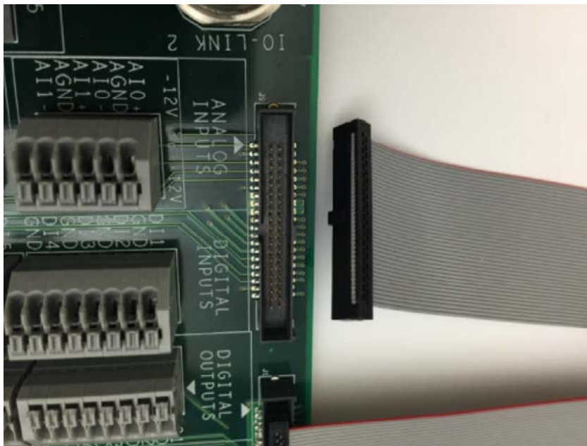
Figure 6. Connecting Cable Assembly to MAXREFDES150ATACH#.
